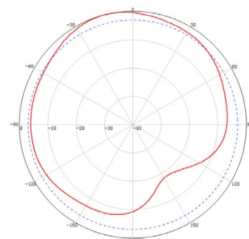
E Plane
