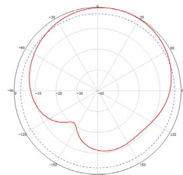
H Plane
