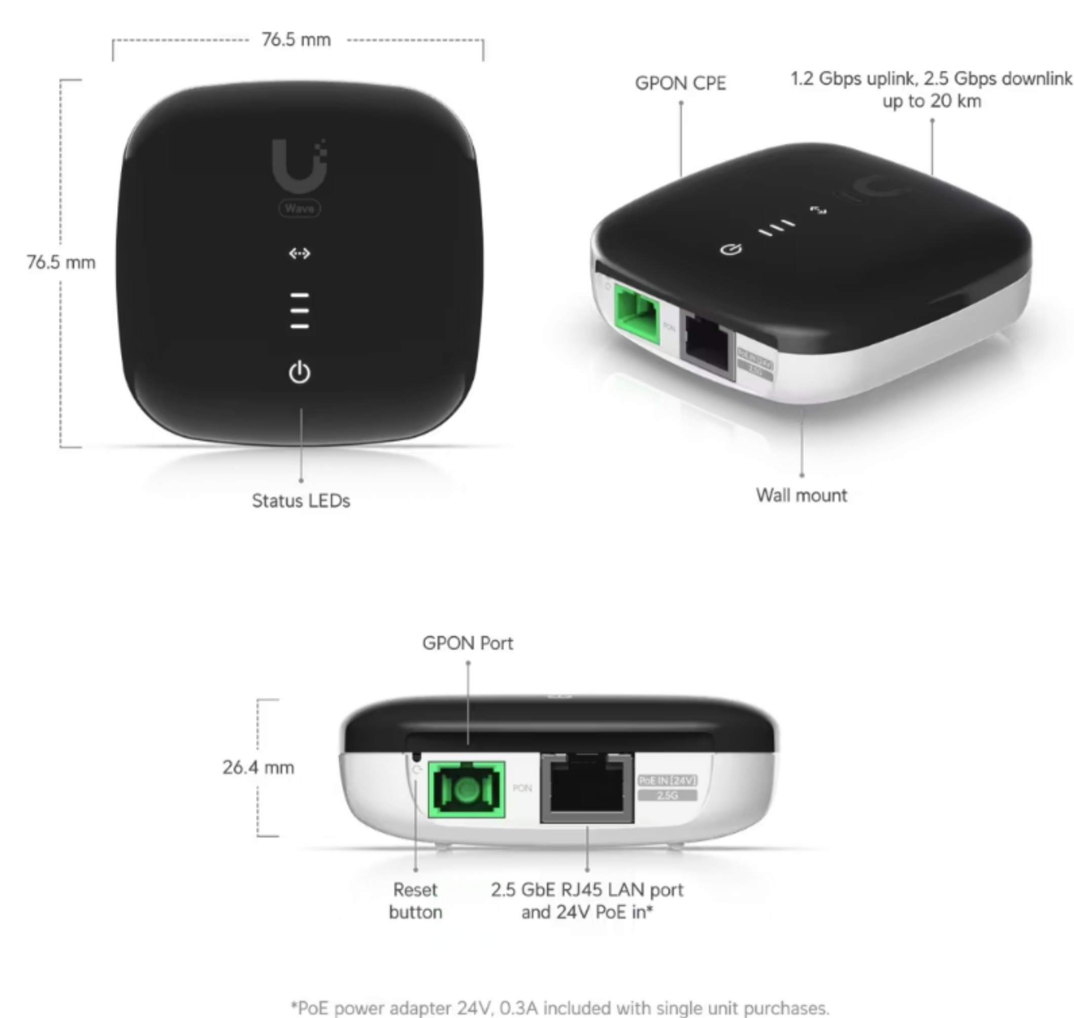
*PoE power adapter 24V, 0.3A included with single unit purchases.
